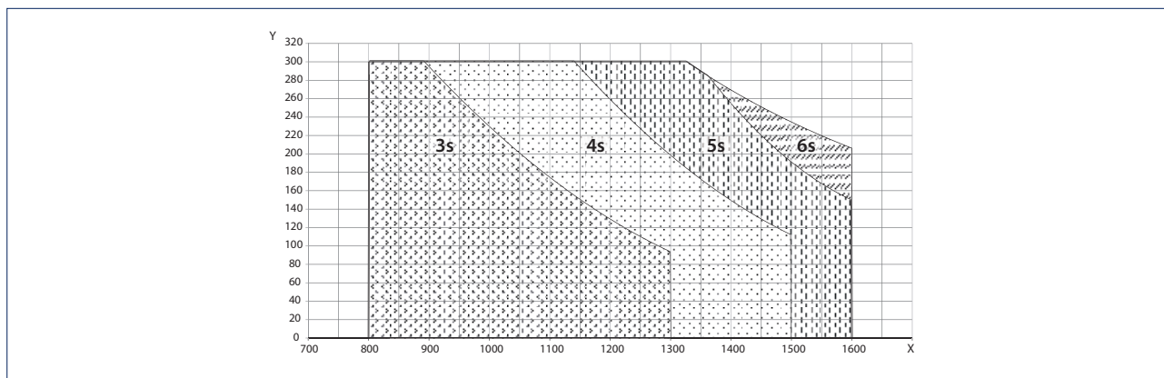
Diagram showing the use of Powerturn with opening times of up to 90° door opening angle
